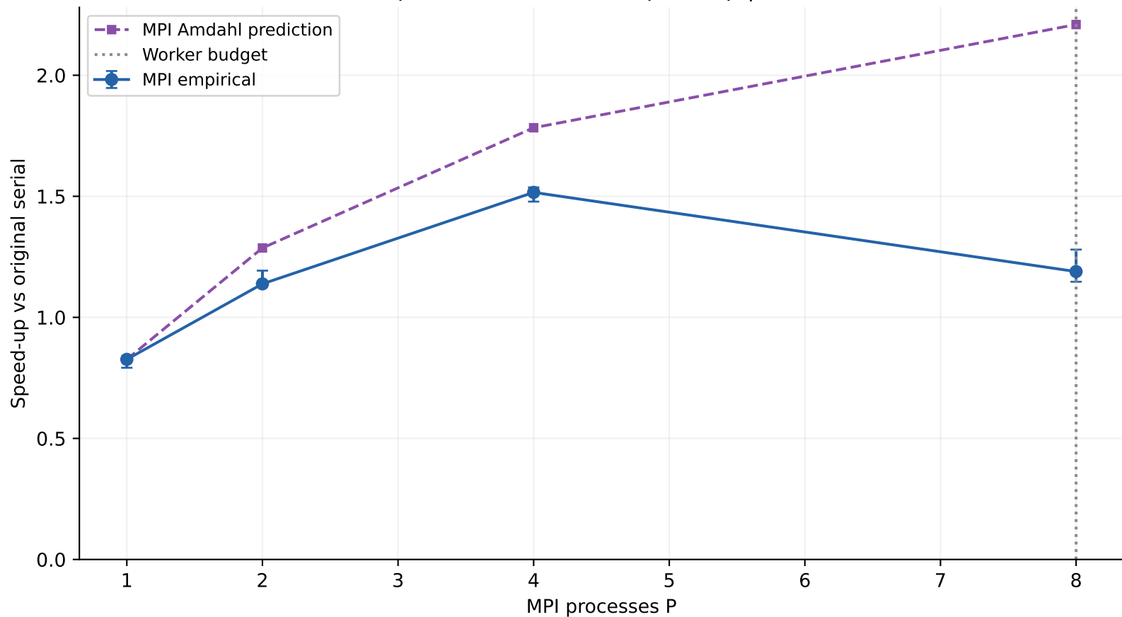
6. MPI: empirical vs theoretical speed-up | n=10,000,000
